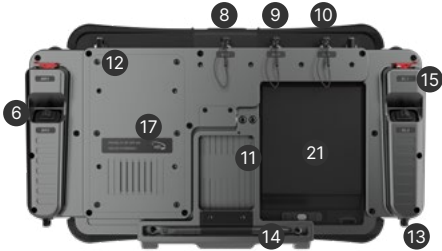
REAR VIEW
